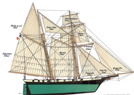
LA RECOUVRANCE 1817
